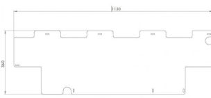
Nirosta Plate No.4 BTM SMALL
